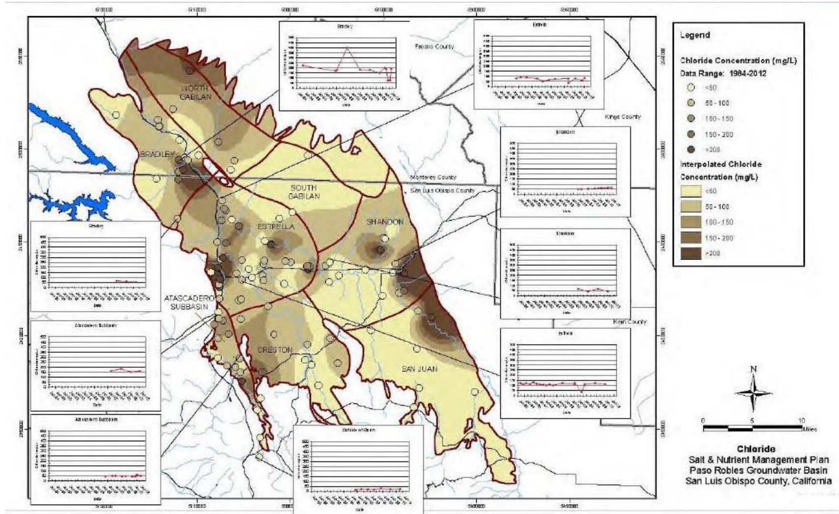
Figure 5-214624. Chloride Regional Distribution and Trends
