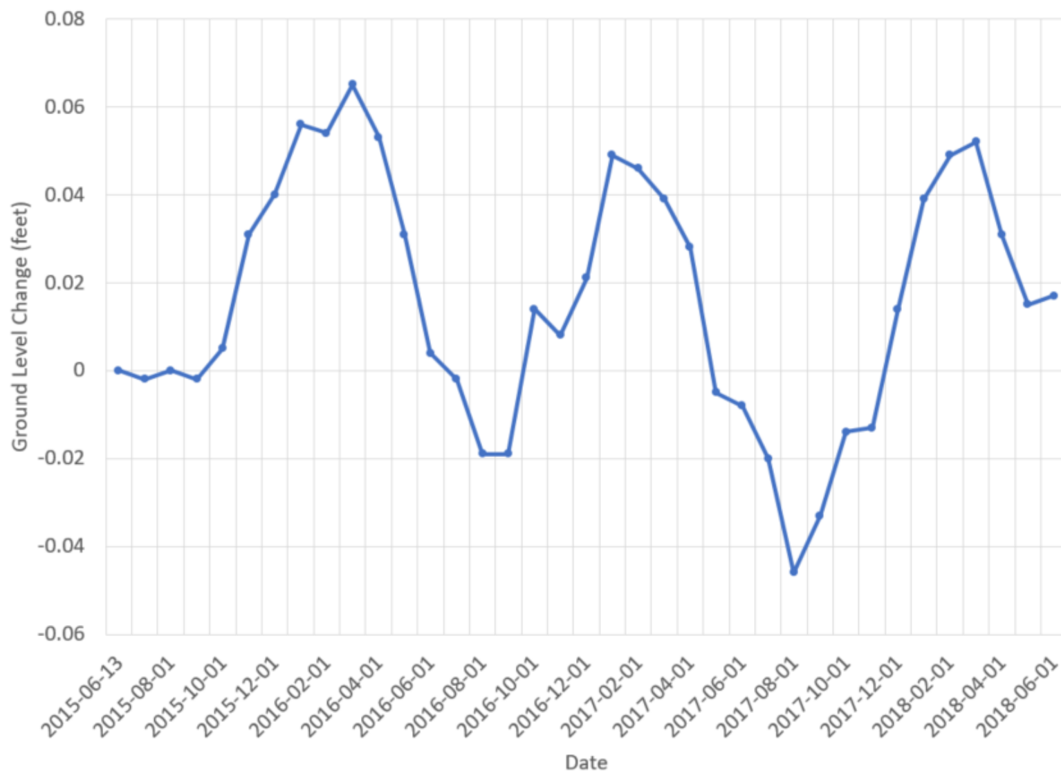
Figure 8-343: Example Seasonal Ground Surface Change
