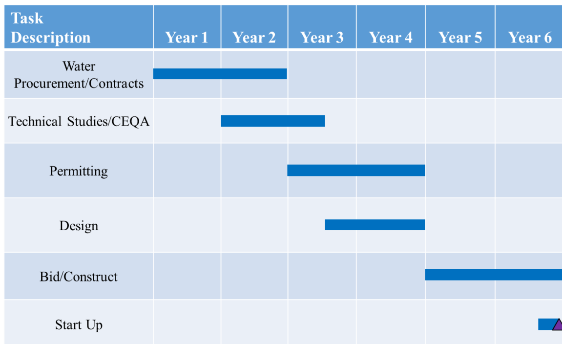
Figure 9-10. Implementation Schedule for NWP Delivery at Salinas and Estrella River Confluence
