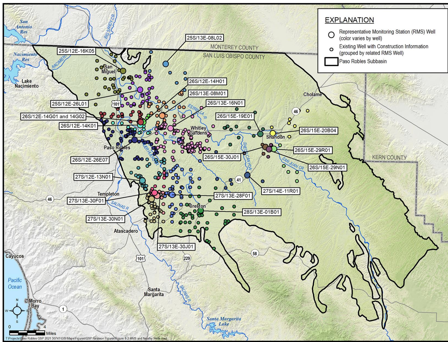
Figure 8-2. Representative Monitoring System (RMS) Wells and Existing Wells with Construction Information
