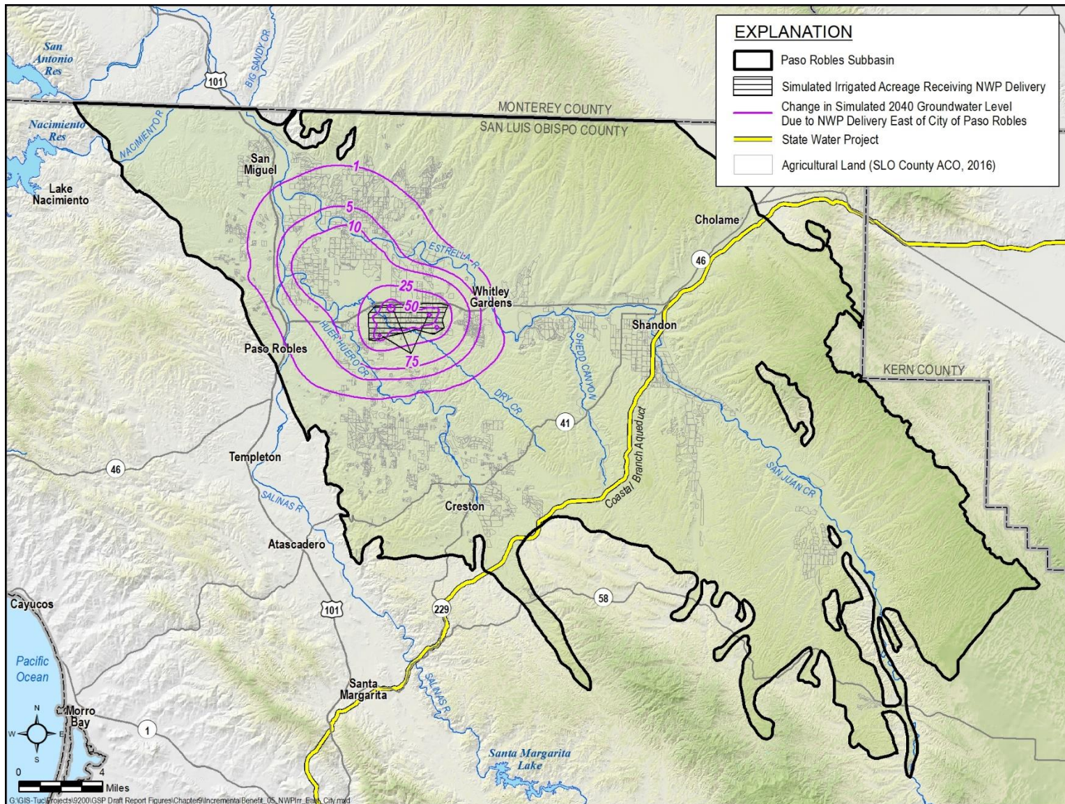
Figure 9-15. Groundwater Level Benefit from NWP Delivery East of City of Paso Robles
