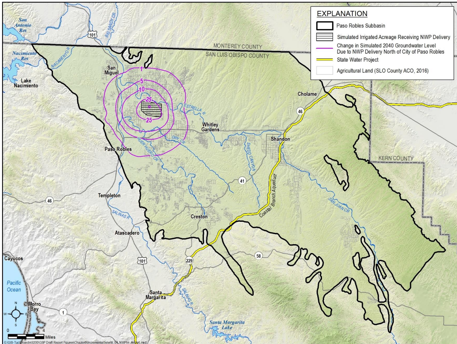
Figure 9-12. Groundwater Level Benefit from NWP Delivery North of City of Paso Robles
