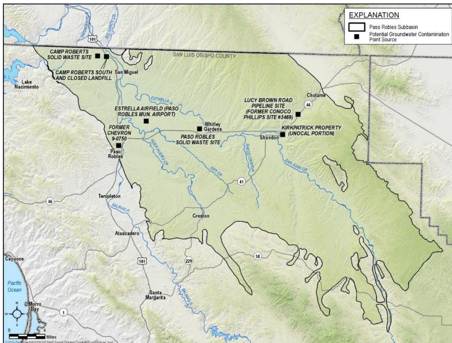
Figure 5-194419. Location of Potential Point Sources of Groundwater Contaminants
