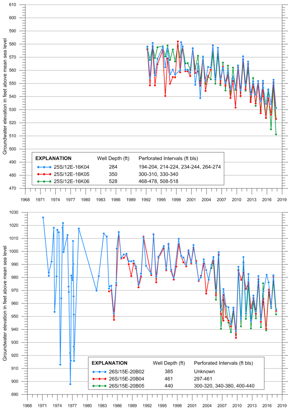
Figure 7-1. Hydrographs of Wells in Well Clusters
