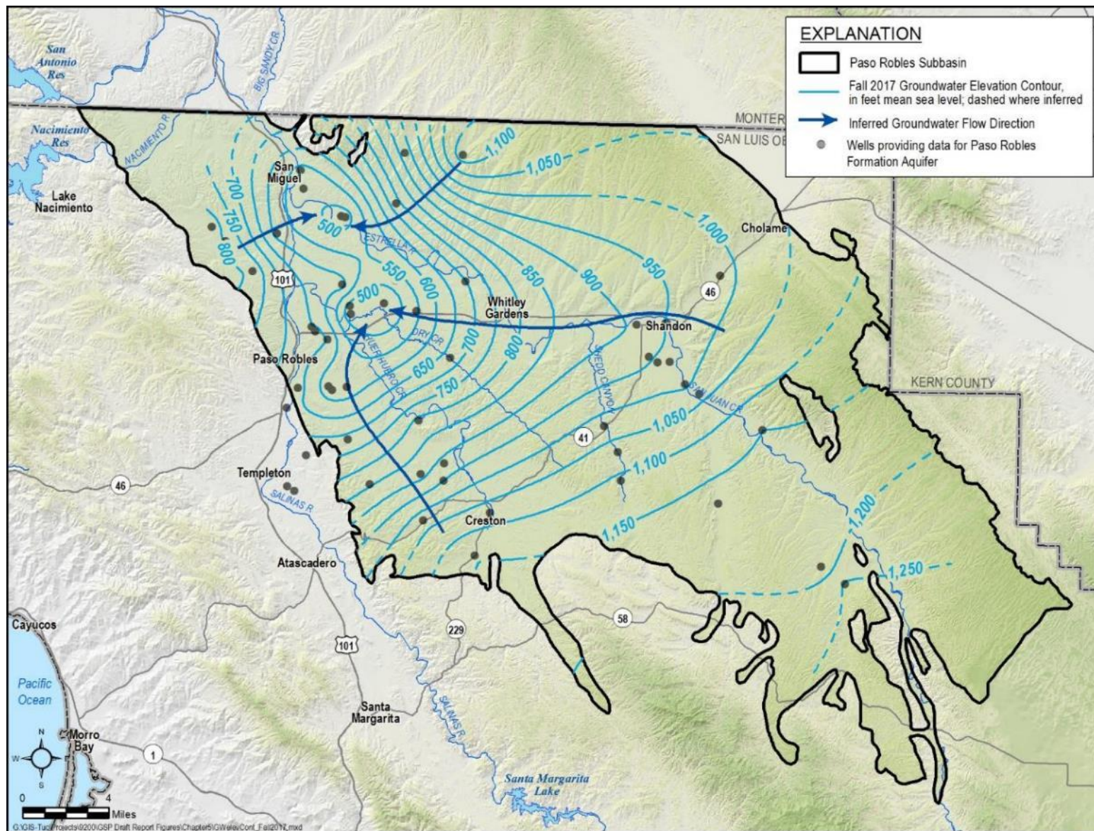
Figure 5-6. Paso Robles Formation Aquifer Fall 2017 Groundwater Elevation Contours
