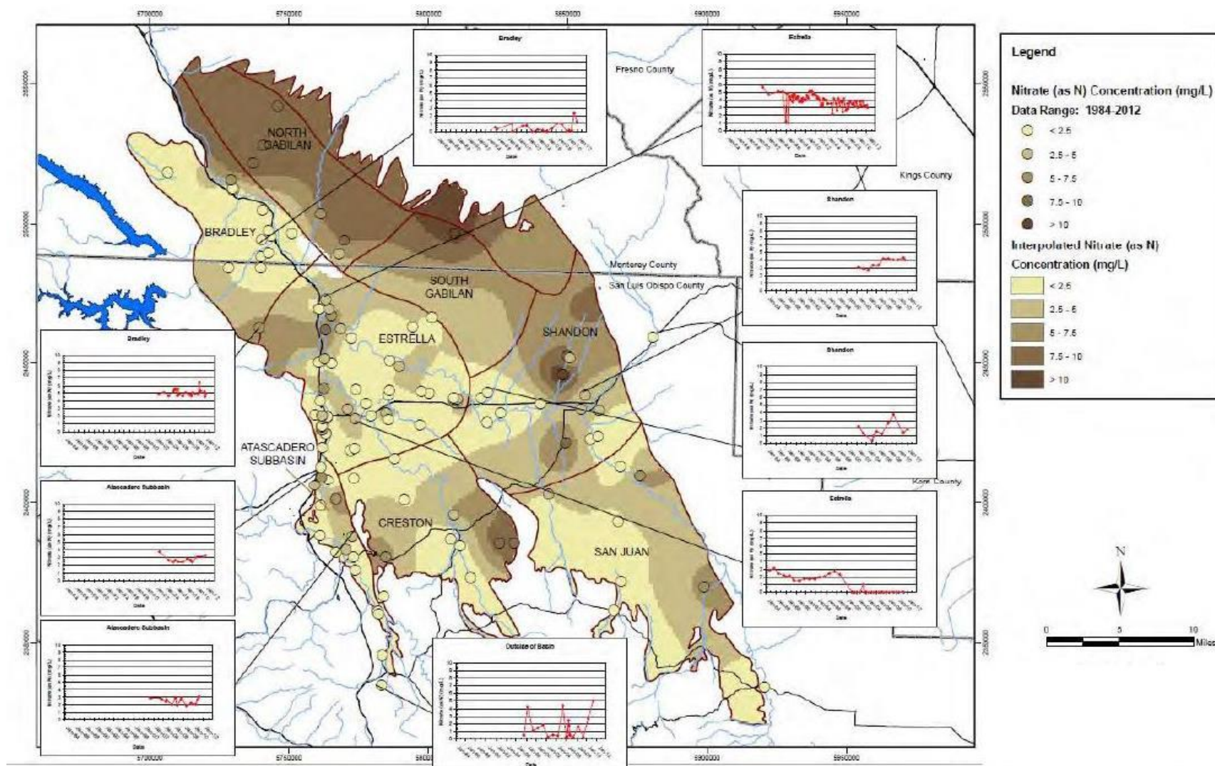
Figure 5-224722. Nitrate Regional Distribution and Trends
