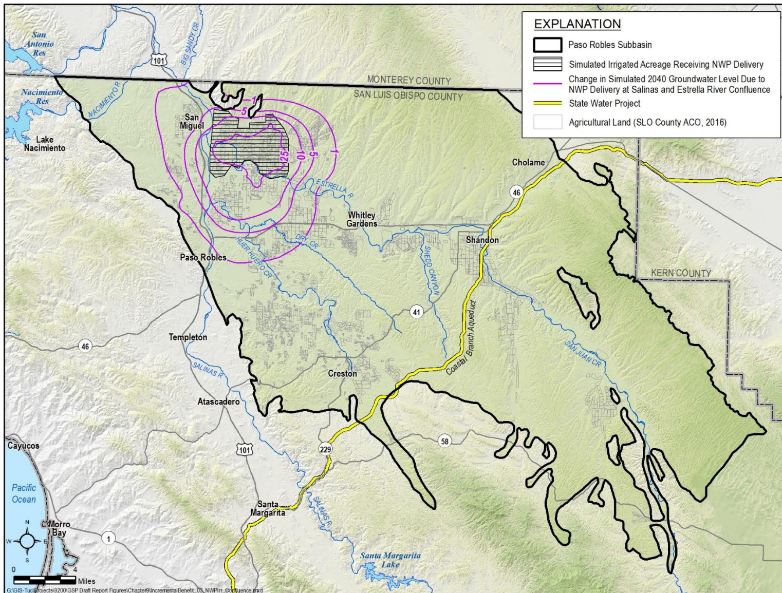
Figure 9-9. Groundwater Level Benefit of NWP Delivery at Salinas and Estrella River Confluence
