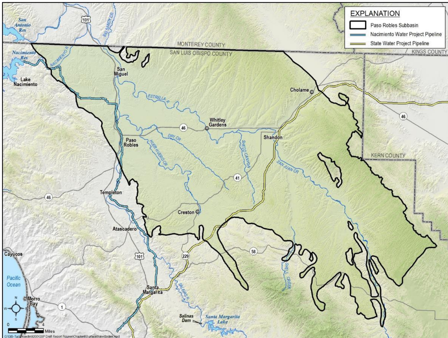
Figure 4-18-18. Surface Water Bodies
