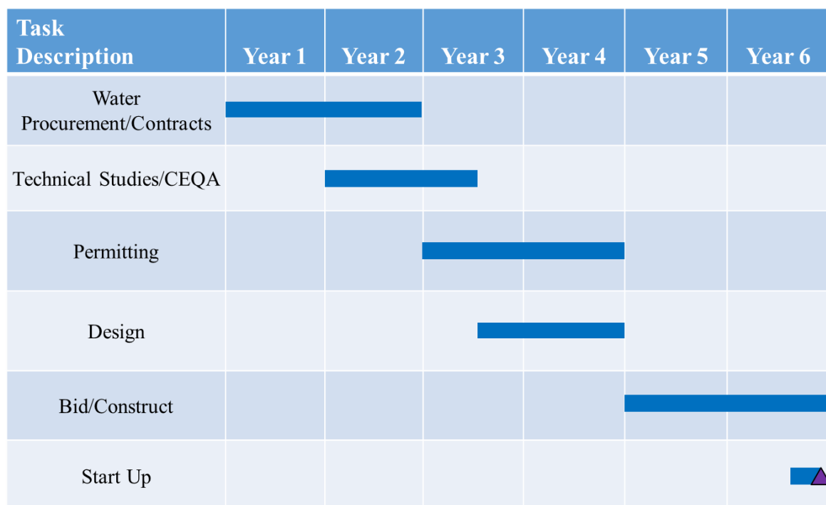
Figure 9-13. Implementation Schedule for NWP Delivery North of City of Paso Robles
