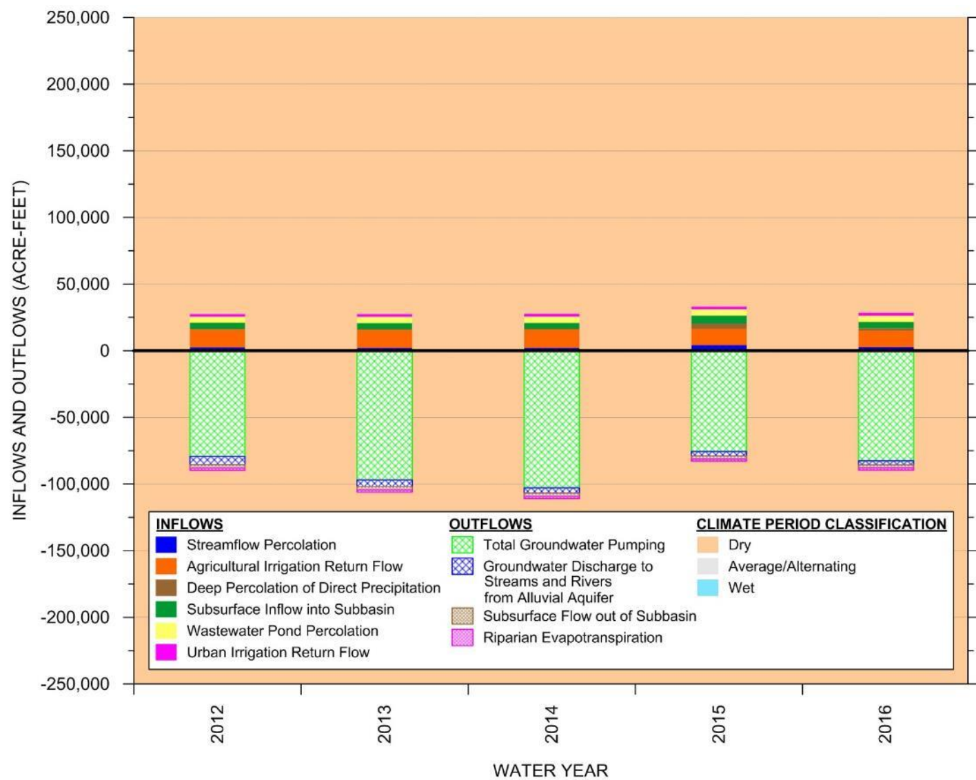
Figure 6-6. Current (2012-2016) Groundwater Inflows and Outflows
