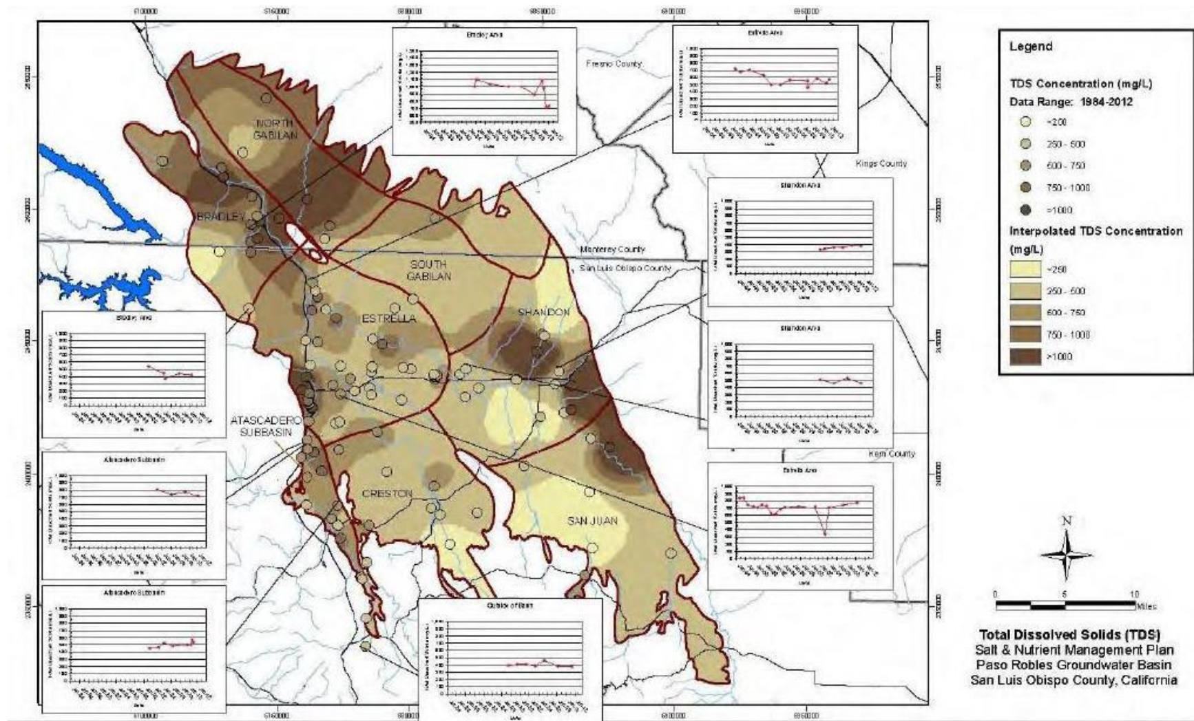
Figure 5-201520. TDS Regional Distribution and Trends
